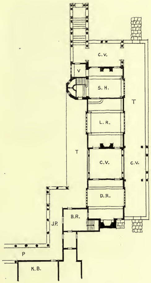
FIRST FLOOR PLAN. House of Mr. Chas. L. Hutchinson.
